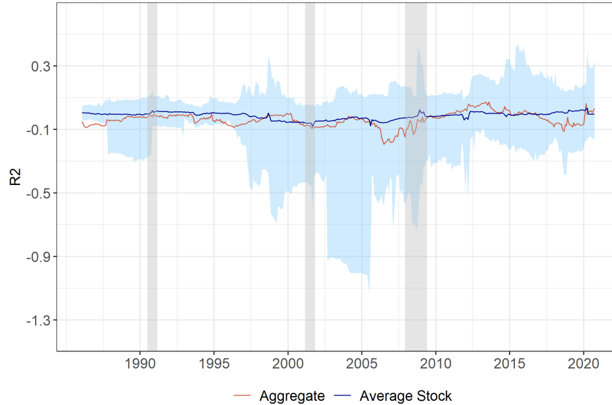
Figure 9: Macro-Raw Predictability series and averaged Individual Raw Predictability
