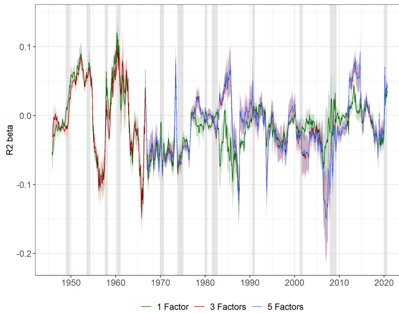
Figure 13: \overline{R^2}_{i,\beta,t} with different Factor Specifications
