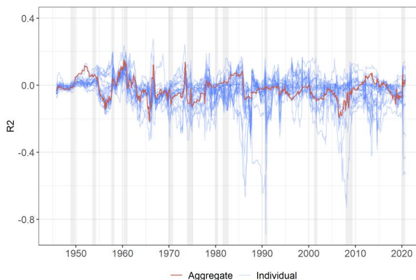
Micro- and Macro-Raw Predictability series, over time
