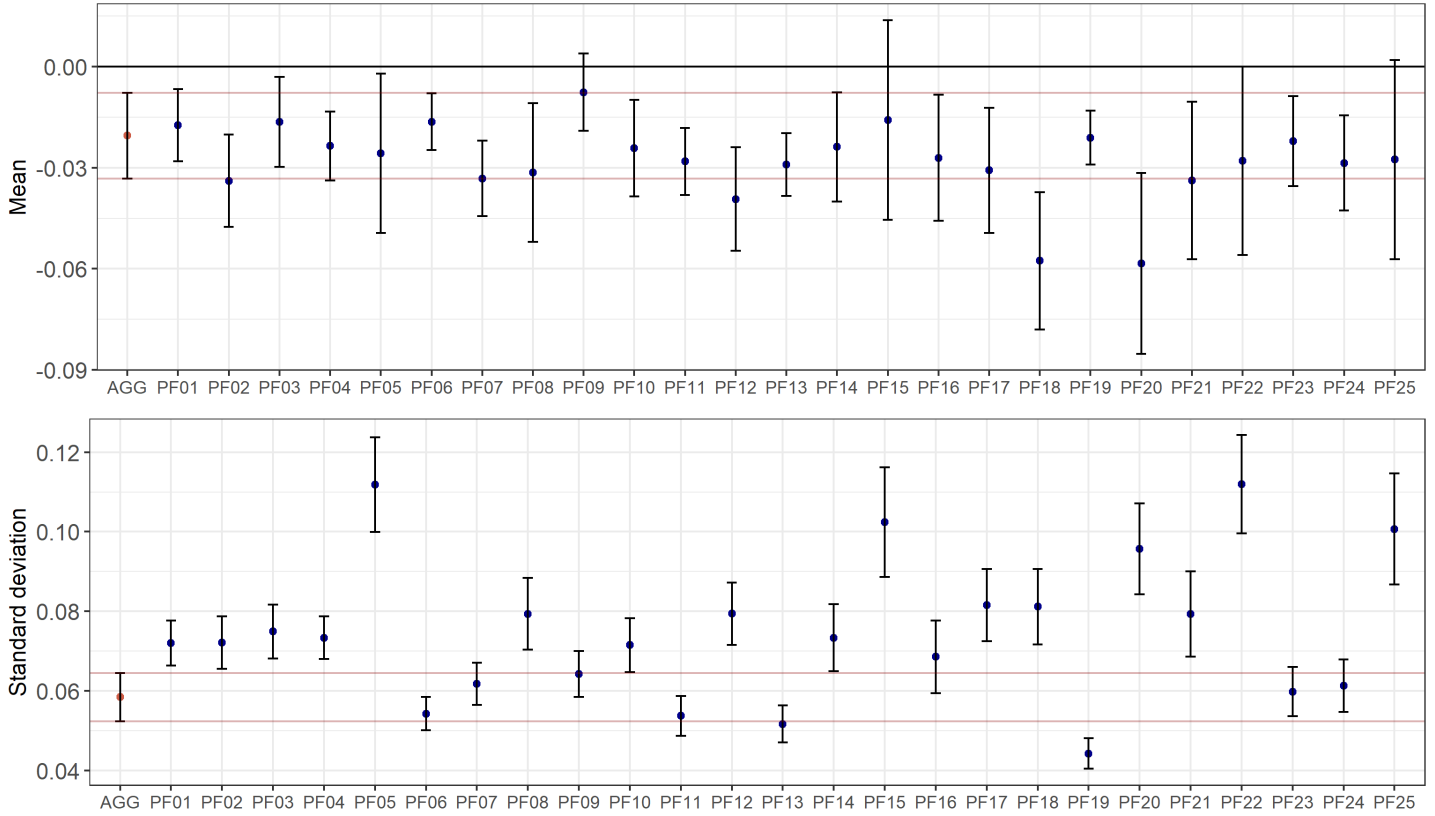
Figure 8: Mean and standard deviations of raw predictability series: confidence intervals
