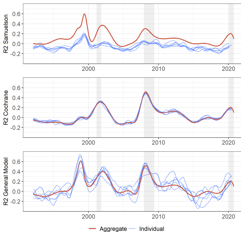
Figure 1: Hypothetical Micro- and Macro-Predictability according to the different views
