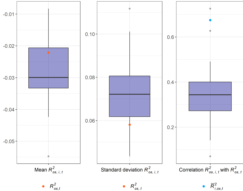
Figure 7: Distribution of Micro-Raw Predictability Statistics
