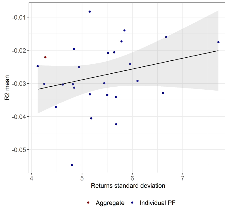
Figure 10: Raw Predictability levels vs. Returns standard deviations
