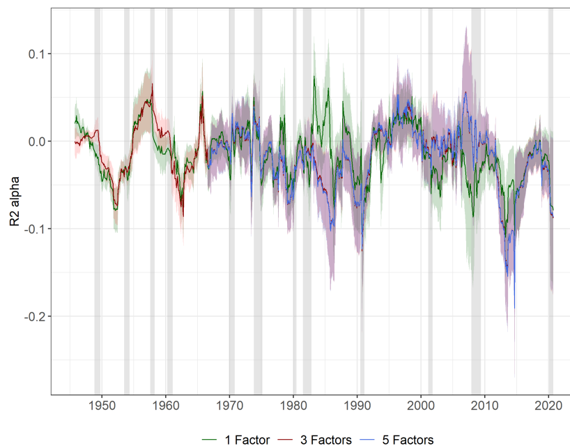
Figure 12: \overline{R^2}_{i,\alpha,t} with different Factor Specifications
