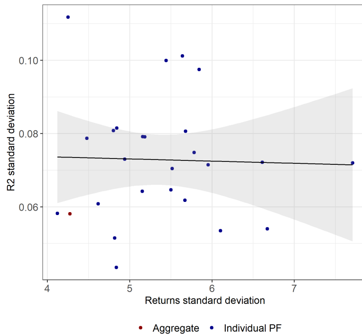
Figure 11: Raw Predictability standard deviations vs. Returns standard deviations
